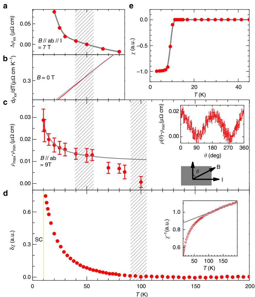
Figure 4 | Magnetoresistivity and susceptibility features of LiTi 2 O 4 thin films. (a) Temperature-dependent longitudinal magnetoresistivity ( B // ab plane/ I ), \Delta\rho_{xx} = \rho_{xx}(B) - \rho_{xx}(0T) , is replotted to demonstrate the crossover temperature (also see Fig. 3b). (b) d\rho_{xx}/dT in zero field. It deviates from the Fermi liquid behaviour, d\rho_{xx}/dT \sim T (grey line), at lower temperatures. (c) Twofold symmetry of in-plane ( ab plane) resistivity, where \rho_{max} ( \theta = 90^\circ ) and \rho_{min} ( \theta = 0^\circ ) are found from plots such as indicated in the inset. The inset shows a typical twofold symmetry at 30 K and 9 T against \theta , which is the angle between the normal direction to current and the field. The error bars are maximum data noise as seen in the inset. (d) The susceptibility with field cooling (1,000 Oe, B // ab plane) shows a Curie-Weiss behaviour at high temperature (see inset \chi^{-1}(T) ). We plot the residual susceptibility \delta\chi as a function of temperature after subtracting the paramagnetic contribution. The \delta\chi starts to increase below 100 \pm 10 K, coincident with the starting temperature of the twofold symmetry of in-plane resistivity. (e) The susceptibility with zero-field cooling shows a good superconducting screening signal, suggesting our LTO films are of high quality. The shading areas around 100 K and 50 K represent the uncertainties in defining the starting point of the anisotropic AMR and the abrupt increase, respectively.
