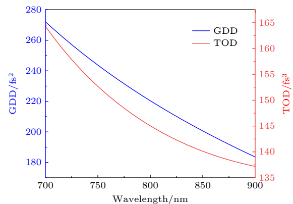
图 2 H-ZF52A 材料引入的二、三阶色散分布曲线 Fig. 2. Second and third order dispersion introduced by H-ZF52A material.
